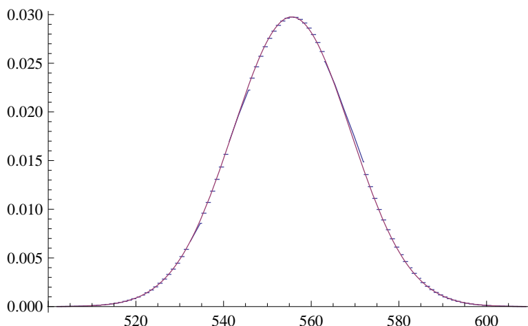
FIGURE 1. Plot of the probability p_{2010}(k) of having exactly k + 1 summands in the Zeckendorf decompositions of integers in [\mathcal{F}_{2010}, \mathcal{F}_{2011}) (with p_n(k) = \binom{n-1-k}{k} / \mathcal{F}_{n-1} ) against the Gaussian with mean \mu_{2010} \approx 555.55 and variance \sigma_{2010}^2 \approx 179.78 .
